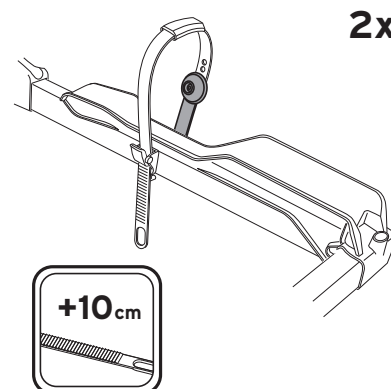
3. Extension strap kit Art. 37661
